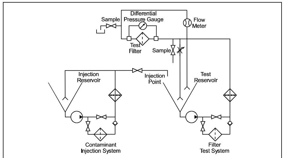
Figure 3 Schematic of Multipass Filter Test System
