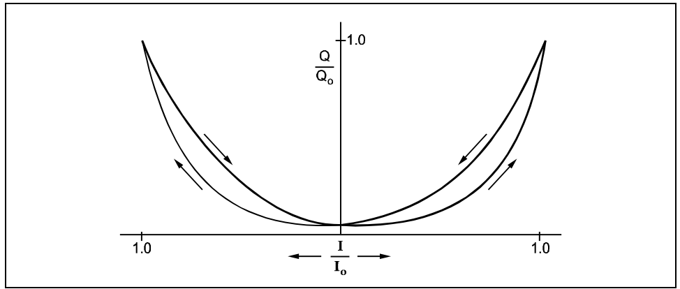
Figure 11 Servovalve Performance in Clean Oil
